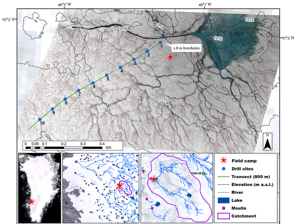
Figure 2. Ortho-rectified image mosaic of the study area at 6 cm ground resolution from RGB camera imagery collected 10 July 2016 on board a quadcopter drone. Background 30 m Landsat image collected same day. Shallow ice cores extracted at 80 m intervals (blue circles) along the 800 m transect provide ice density measurements to depths of 1.1 m, with two additional shallow ice cores extracted to 1.8 m depth at interval 1. Insets (below) show the 63.1 km 2 supraglacial catchment extent (magenta outline), as delineated from WorldView satellite stereo-photogrammetric digital elevation model topography, and supraglacial river and moulin locations derived from Landsat 8 imagery (Yang and Smith, 2016).
