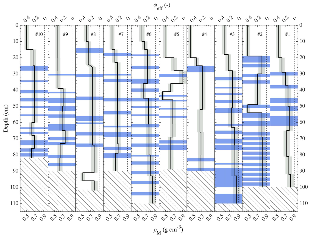
Figure 4. Subsurface measured ice density ( \rho_M ) and corresponding calculated effective porosity ( \phi_{\text{eff}} ), and stratigraphy profiles from 10 shallow ice cores (#10–1, left to right) extracted at 80 m intervals along the study transect (see Fig. 2 for ice core locations). Horizontal blue shading represents solid ice layers. Vertical dashed line at solid ice density 0.917 \text{ g cm}^{-3} . Assumed \pm 10\% measurement uncertainty represented by shaded grey bars. Hatched areas are no data.
