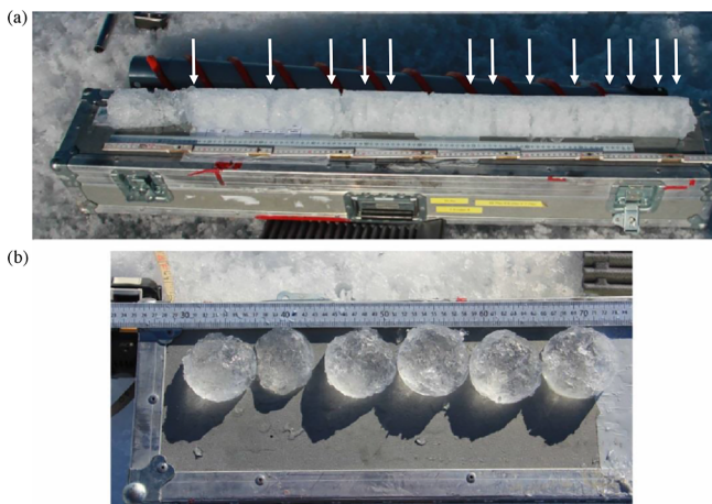
Figure 5. (a) Typical near-surface shallow ice core (core #6) prior to in situ analysis of density and stratigraphy. Clear, solid ice lenses alternate with granular, fractured ice. Approximate locations of ice lenses noted with white arrows (not all lenses are clearly visible). (b) Ice lenses removed and confirmed after completed core analysis (core #1).
