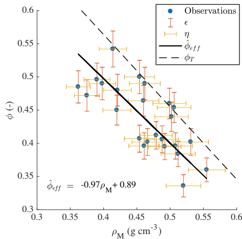
Figure 6. Linear relationship ( \hat{\phi}_{\text{eff}} solid line) between measured ice density ( \rho_M ) and effective porosity ( \phi_{\text{eff}} ) and assumed \pm 10\% measurement error (whiskers). Dashed line is theoretical upper limit where effective porosity equals total porosity (i.e. \phi_T = \rho_M / \rho_T ).
