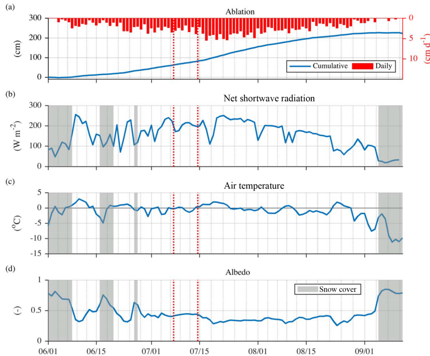
Figure 8. Meteorological records of (a) daily and cumulative ice surface ablation, (b) net shortwave radiation, (c) 2 m air temperature, and (d) albedo, for the period 1 June 2016–15 September 2016. Data were collected by the PROMICE/GAP KAN-M automatic weather station (see Fig. 2 for location). Vertical grey shaded bars indicate time periods when albedo was greater than >0.5 , indicating snow cover was likely present. Albedo is calculated from the ratio of outgoing solar radiation to incoming solar radiation measured \sim 2 m above the ice sheet surface at the KAN-M station (available at: www.promice.org ).
