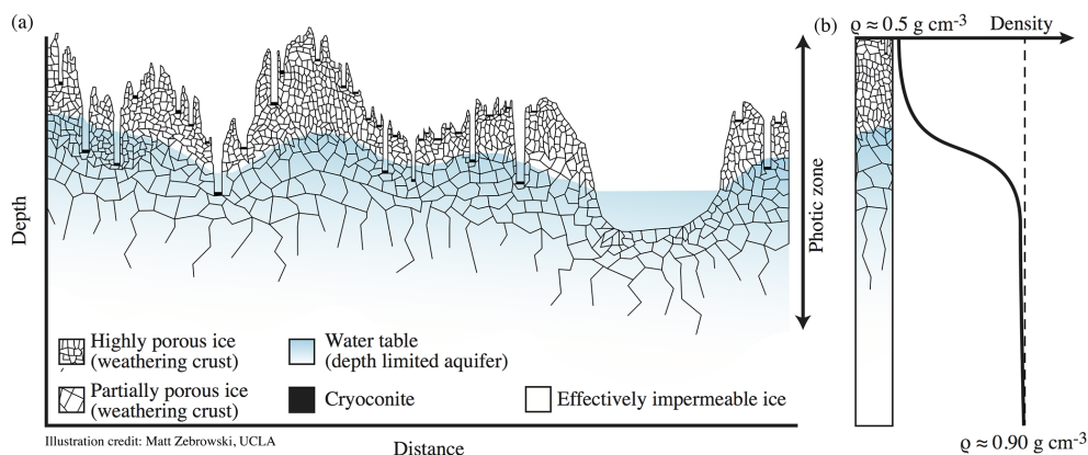
Figure 1. (a) Conceptual diagram of weathering crust structure, highlighting the porous ice layers, cryoconite holes, and saturated water table (adapted from Irvine-Fynn and Edwards, 2014 and Müller and Keeler, 1969). (b) Theoretical subsurface depth-density profile showing the non-linear increase in ice density from the highly porous, low density near-surface ice to higher-density, unweathered glacier ice (adapted from LaChapelle, 1959). Illustration credit: Matt Zebrowski, UCLA.
