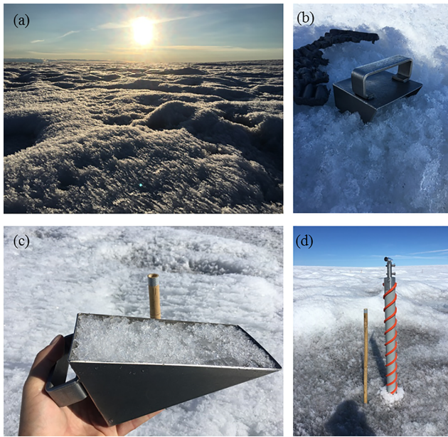
Figure 3. (a) A surface weathering crust was pervasive throughout the study area, characterized by small scale topographic variability and cryoconite holes. (b–c) A 1000 cm 3 steel snow density sampler was vertically inserted into the upper 20 cm weathered ice. (d) A shallow ice corer was used to obtain ice samples to depths of 1.8 m.
