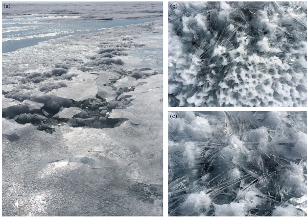
Figure 9. Night-time refreezing of meltwater at the surface of (a) water tracks ( \sim 10 m length scale), and (b) cryoconite holes ( \sim 0.1 – 1 m length scale) was frequently observed during the field study. Photos were collected by the first author during the 6–12 July 2016 field campaign between 04:00 and 07:00 local time.
