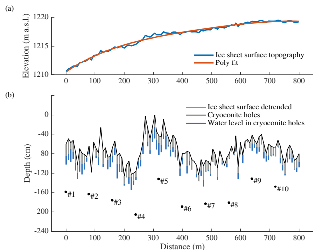
Figure 7. (a) Ice sheet surface topography along the 800 m study transect extracted from a 6 cm resolution stereo-photogrammetric digital elevation model derived from RGB imagery collected 10 July 2016 from a quadcopter drone and the second-order polynomial best fit. (b) Ice sheet surface topography detrended with the polynomial best fit, cryoconite hole depths (vertical grey bars), and cryoconite hole water levels (vertical blue bars) sampled along the 800 m study transect, adjusted to a common vertical reference. Locations of the 10 shallow boreholes and their depth relative to the detrended surface are labelled #1–10.
